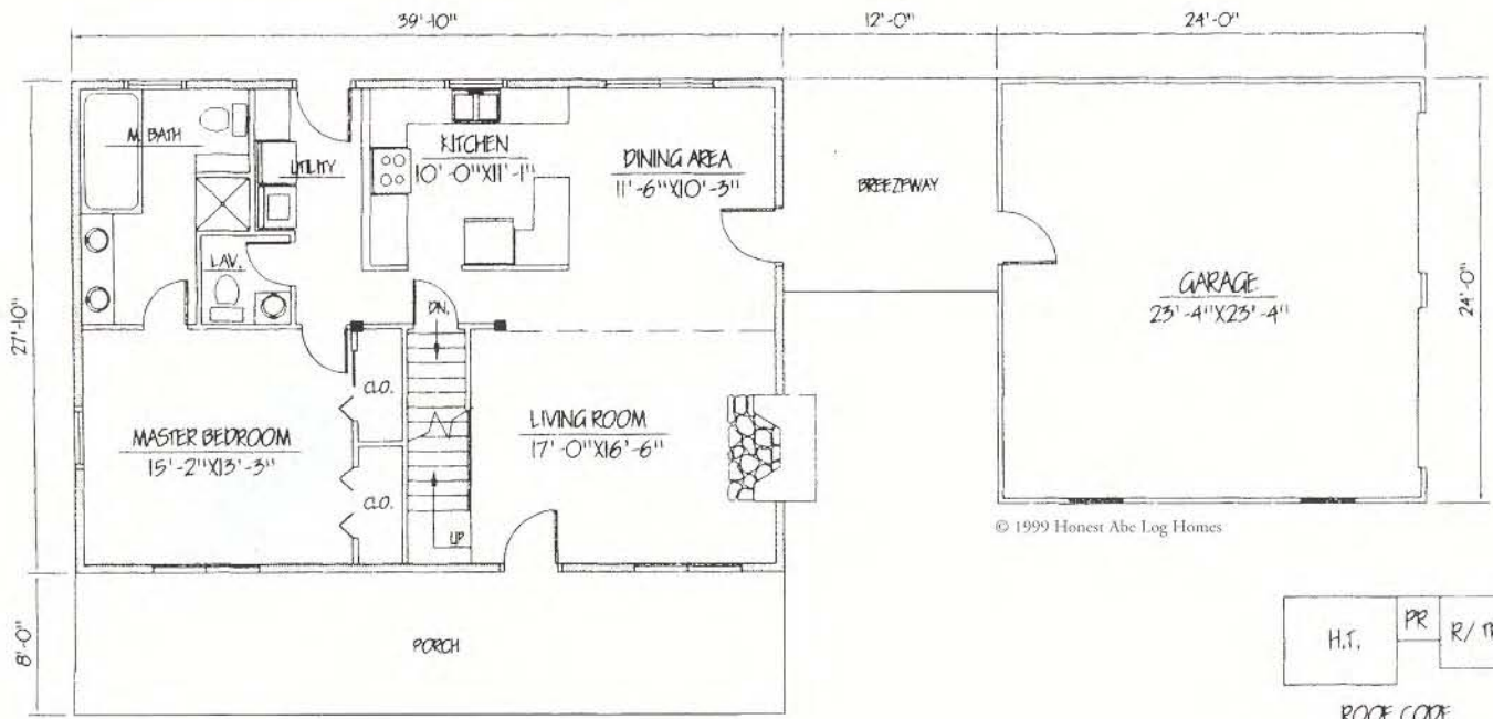
FIRST FLOOR PLAN LAYOUT OPTION 'B'
