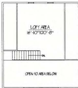
SECOND FLOOR PLAN 892 50. FT.
